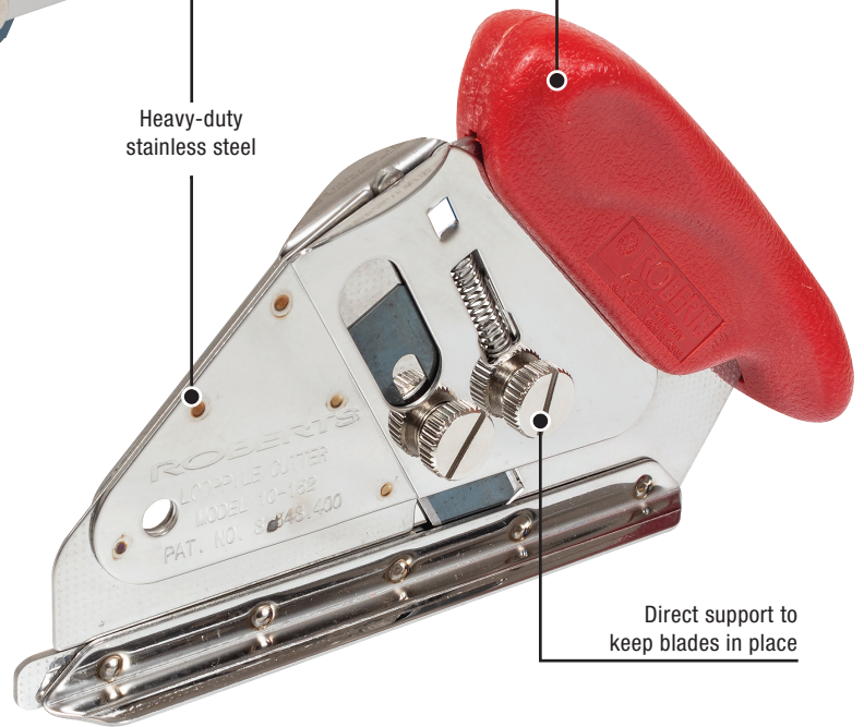
LOOP PILE CUTTER 10-152-3
