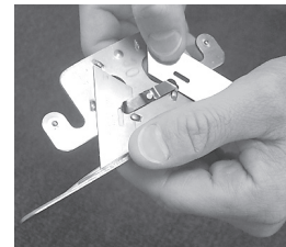
Remove old blades as shown. Insert new blade under spring clip and position between raised guides. When only one end of each blade is dull you need only switch blades to the other position to double the life of the blades. Note: Use only ROBERTS Trimmer Blades in this tool. For satisfactory performance, you must be able to read the printing on the blade, when it is in position.
