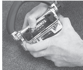
2. Insert locating plate between spacers at the height desired, using the finger notches at either end. The average location will be on top of the fourth spacer. If this leaves the carpet too long move down one or two spaces. If the carpet is too short, move the locating plate, to a higher position.
