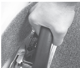
1. Start cut at 45° angle. Moving the trimmer down to a flat position on the floor. It is usually necessary to pull the carpet tight with the other hand when starting the cut.
